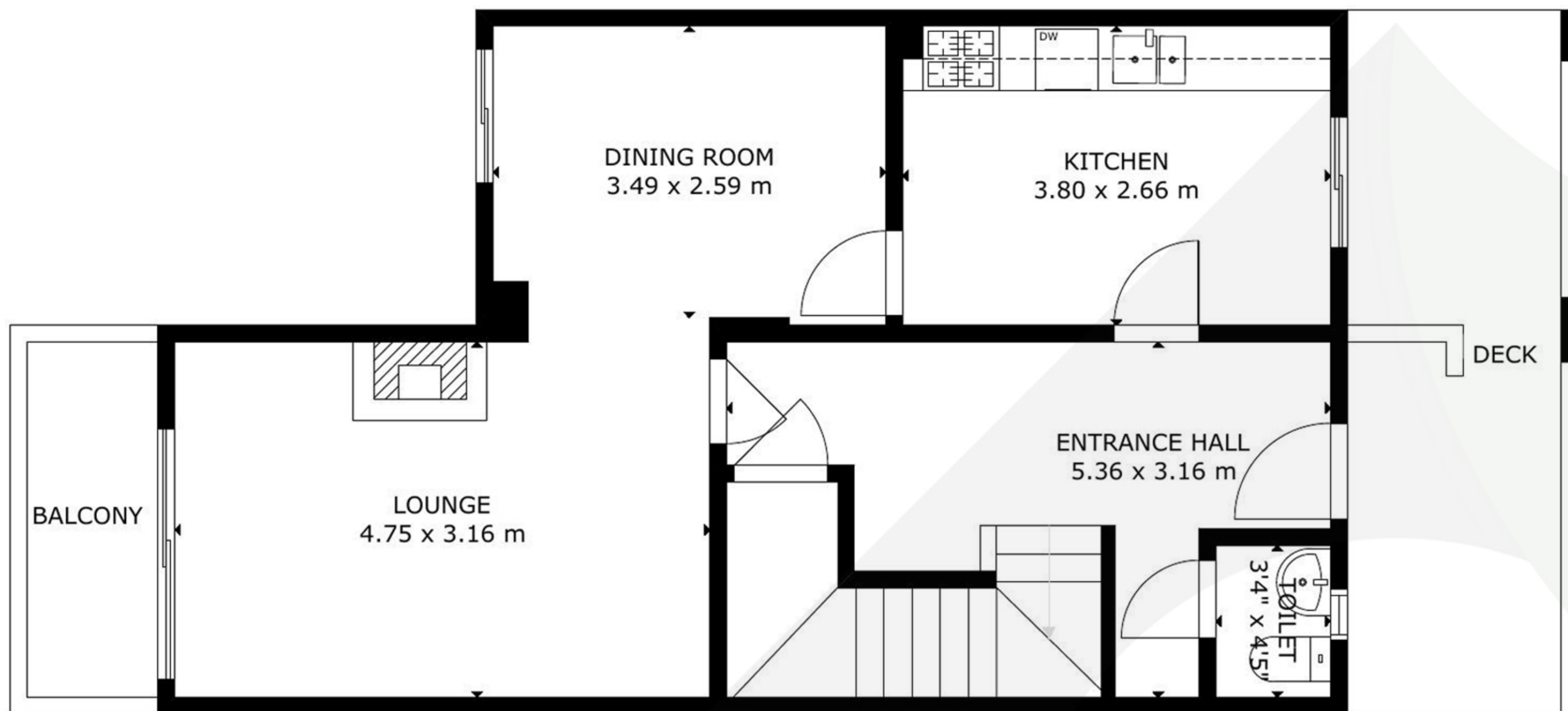
GROUND FLOOR
