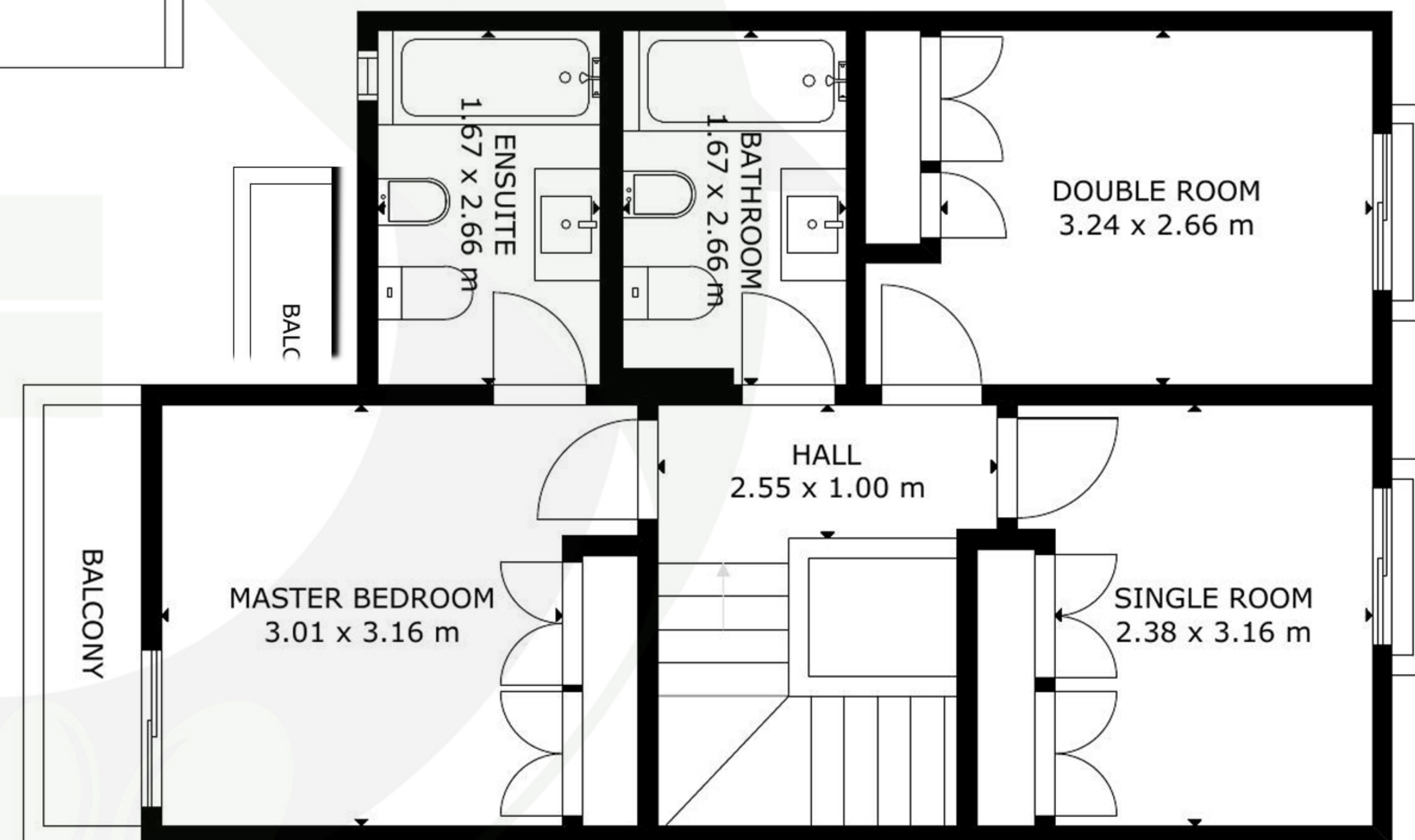
FIRST FLOOR
