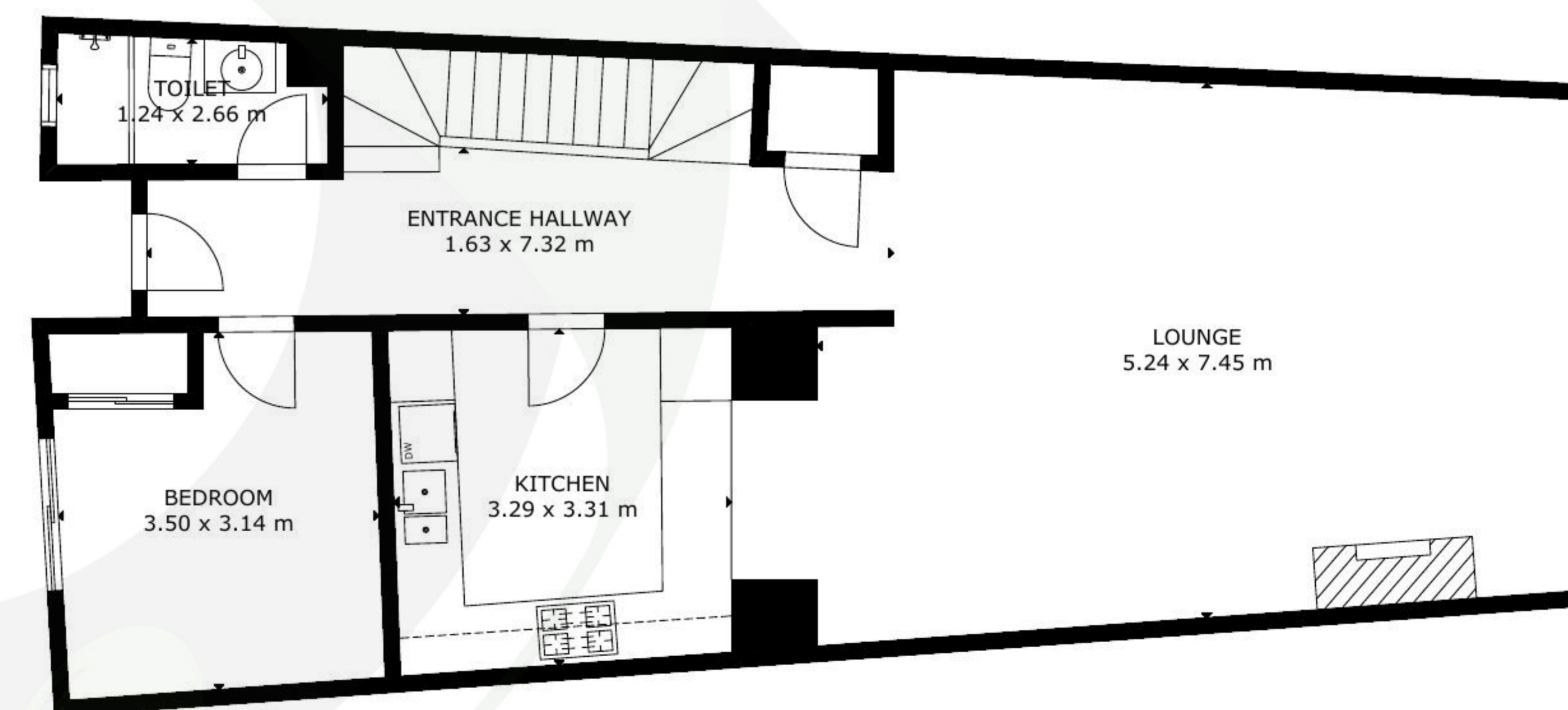
GROUND FLOOR
