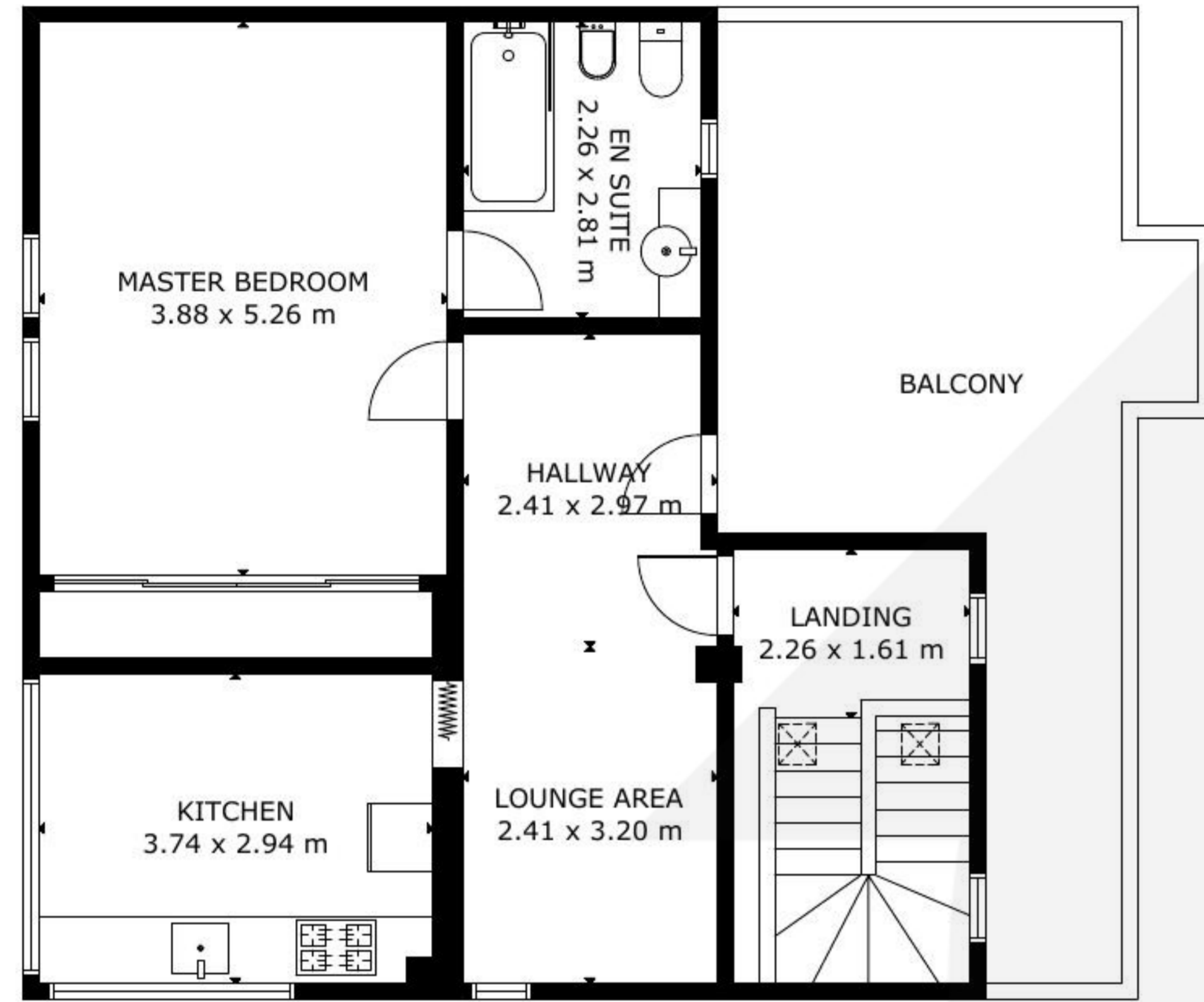
SECOND FLOOR
