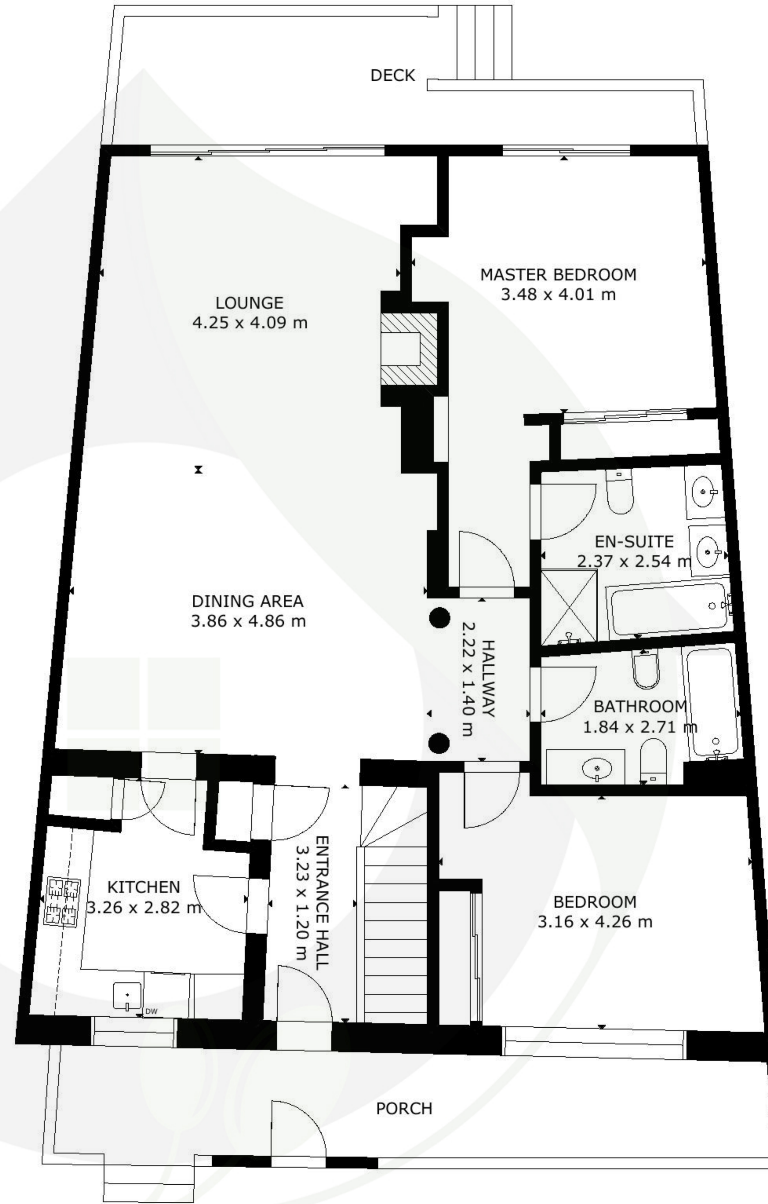
GROUND FLOOR
