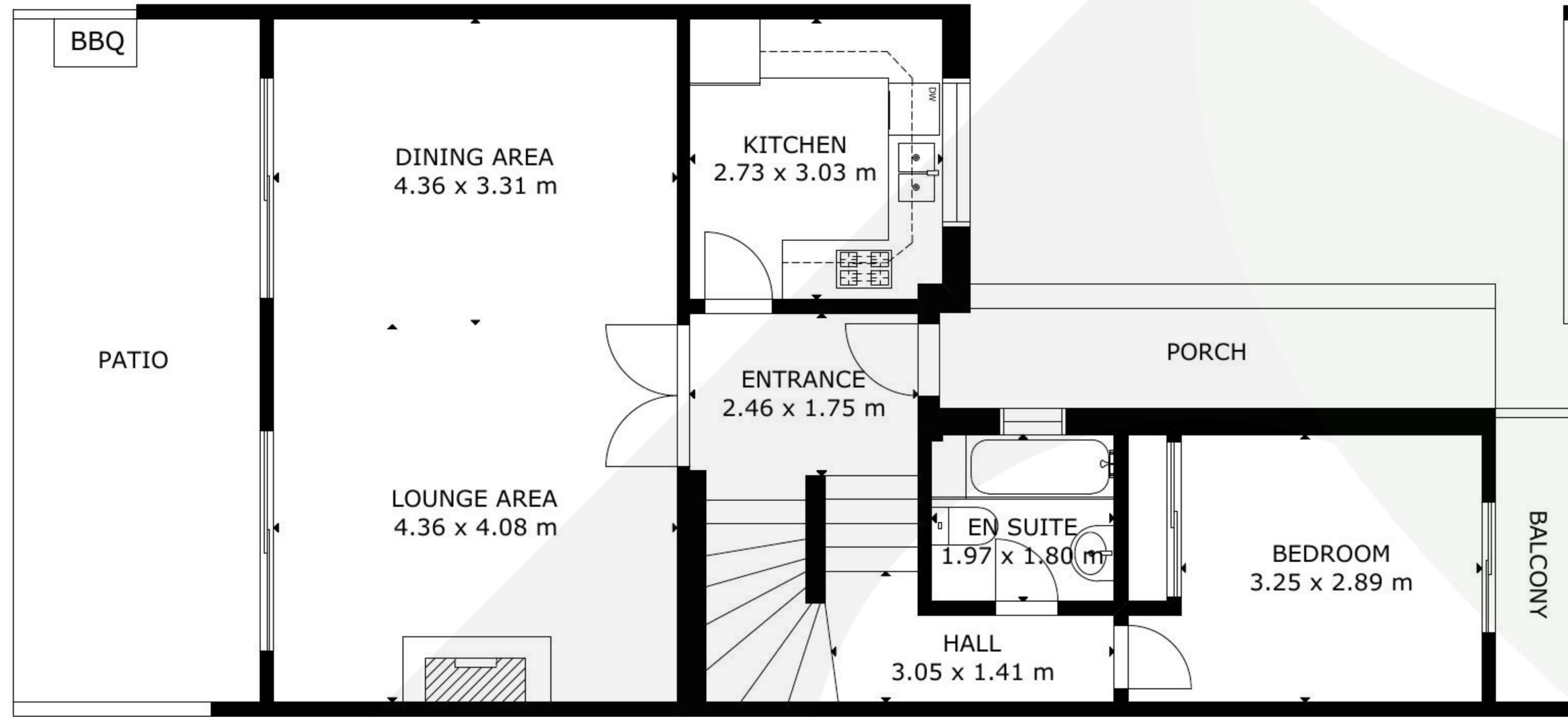
GROUND FLOOR
