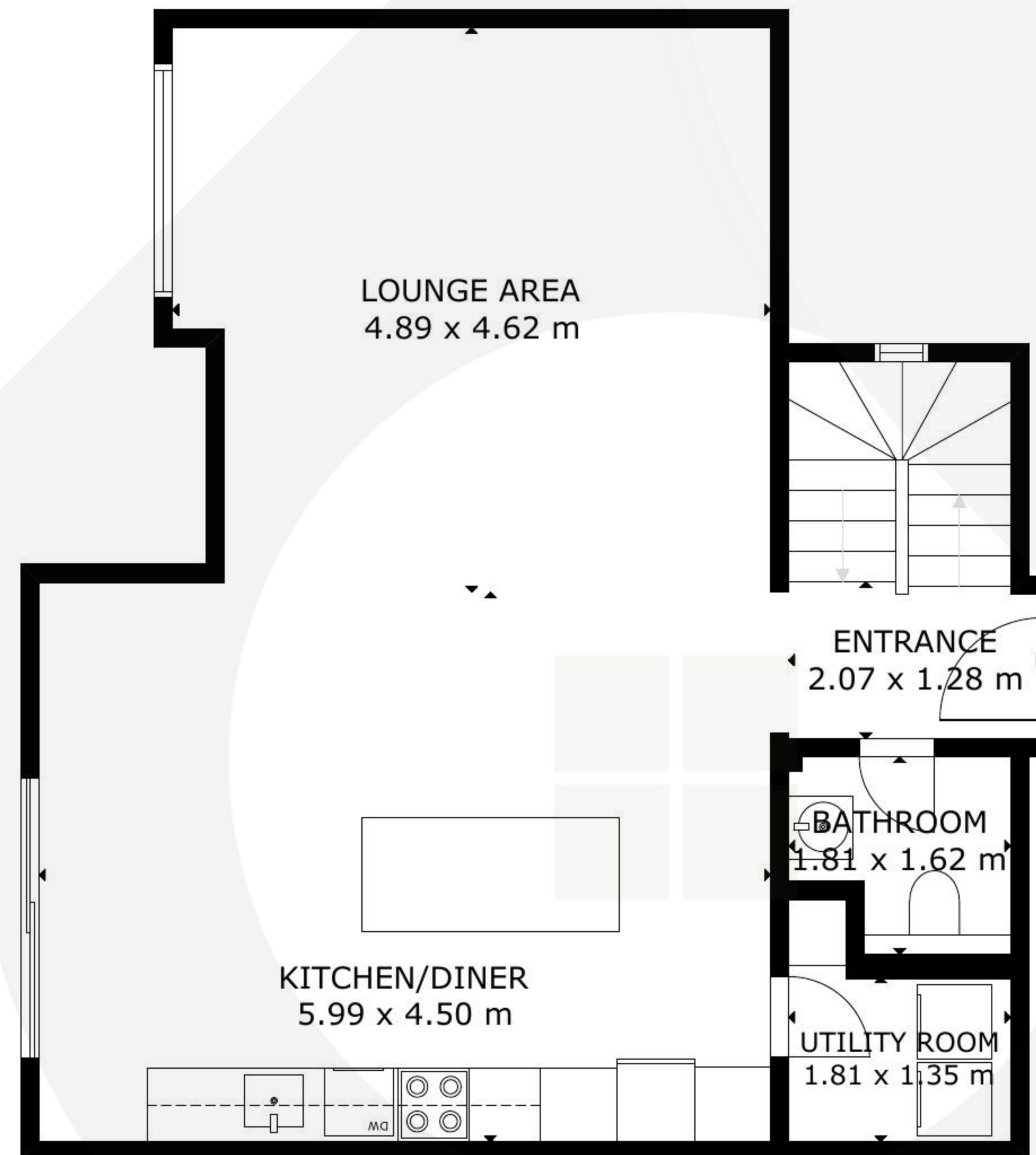
GROUND FLOOR
